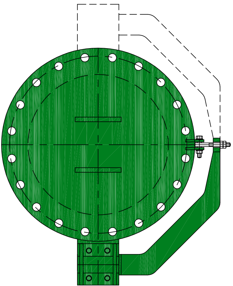
FRONT ELEVATION
